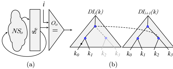
Fig. 1. (a) A common sequential circuit for which deobfuscation can need exponential queries that are exponentially long; (b) DIP conditions in an exponential query scheme have potentially many equivalent nodes.
