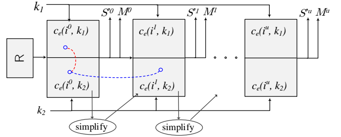
Fig. 2. Iterative unrolling/simplification/termination/settlement-checking. By removing the initialization condition R we can study inductive properties, check for u -round termination, and simplify the transition relation for the next round. Merges between corresponding nodes in the mitter (red and blue dotted-lines) represent settled nodes for which their fanin functions is fully deobfuscated.
